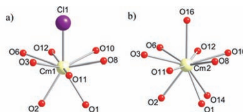
Figure 2. Views of two different coordination environments of \text{Cm}^{\text{III}} sites in \text{Cm}_2[\text{B}_{14}\text{O}_{20}(\text{OH})_7(\text{H}_2\text{O})_2\text{Cl}] with resolved disorder.
